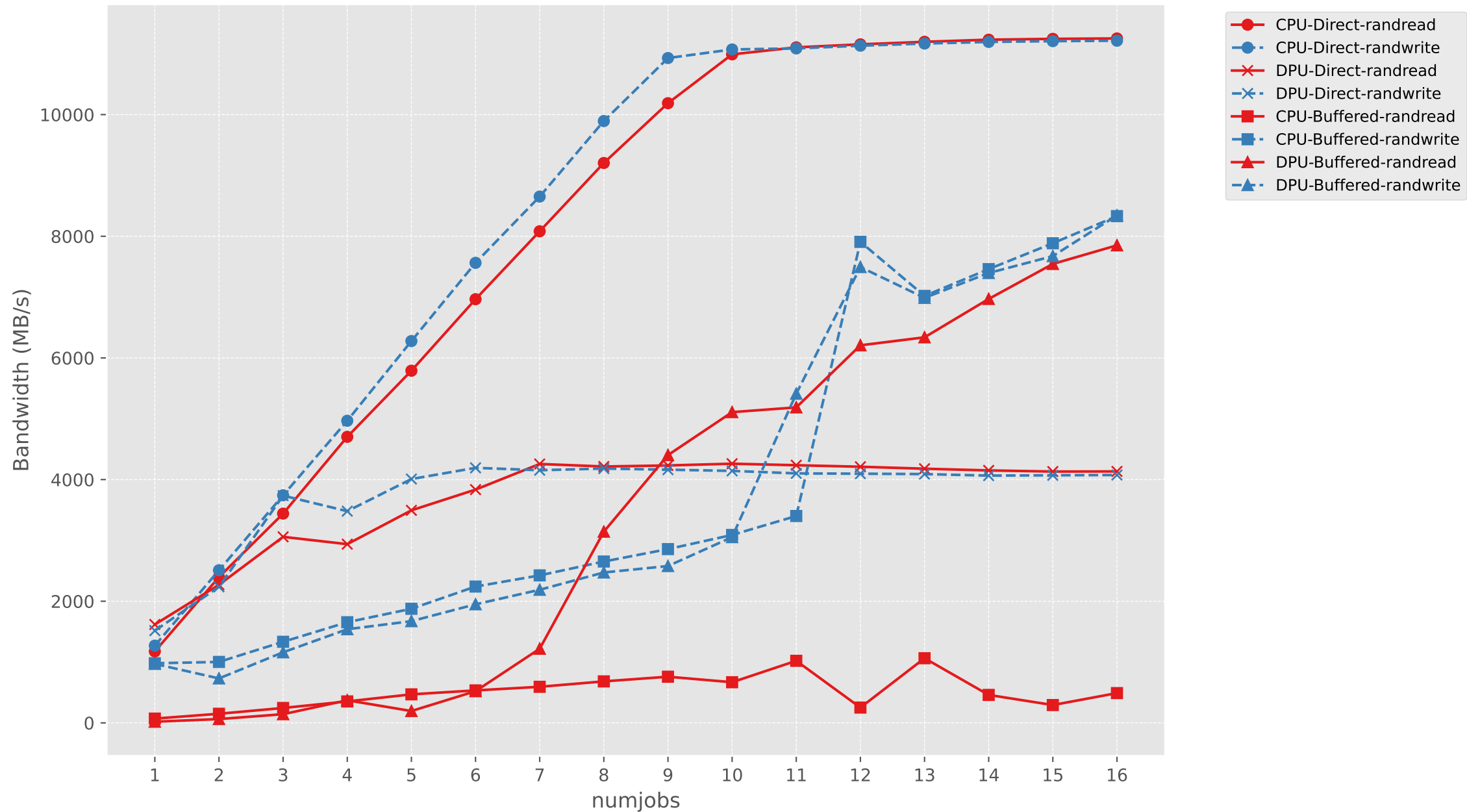
Bandwidth vs numjobs (CPU vs DPU, Direct vs Buffered)
